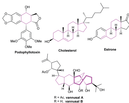
Fig. 13 Several natural products with complex carbocyclic skeletons.
