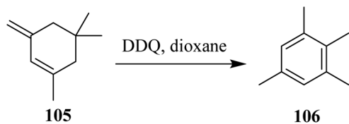
Scheme 42 Aromatization induced by DDQ.
