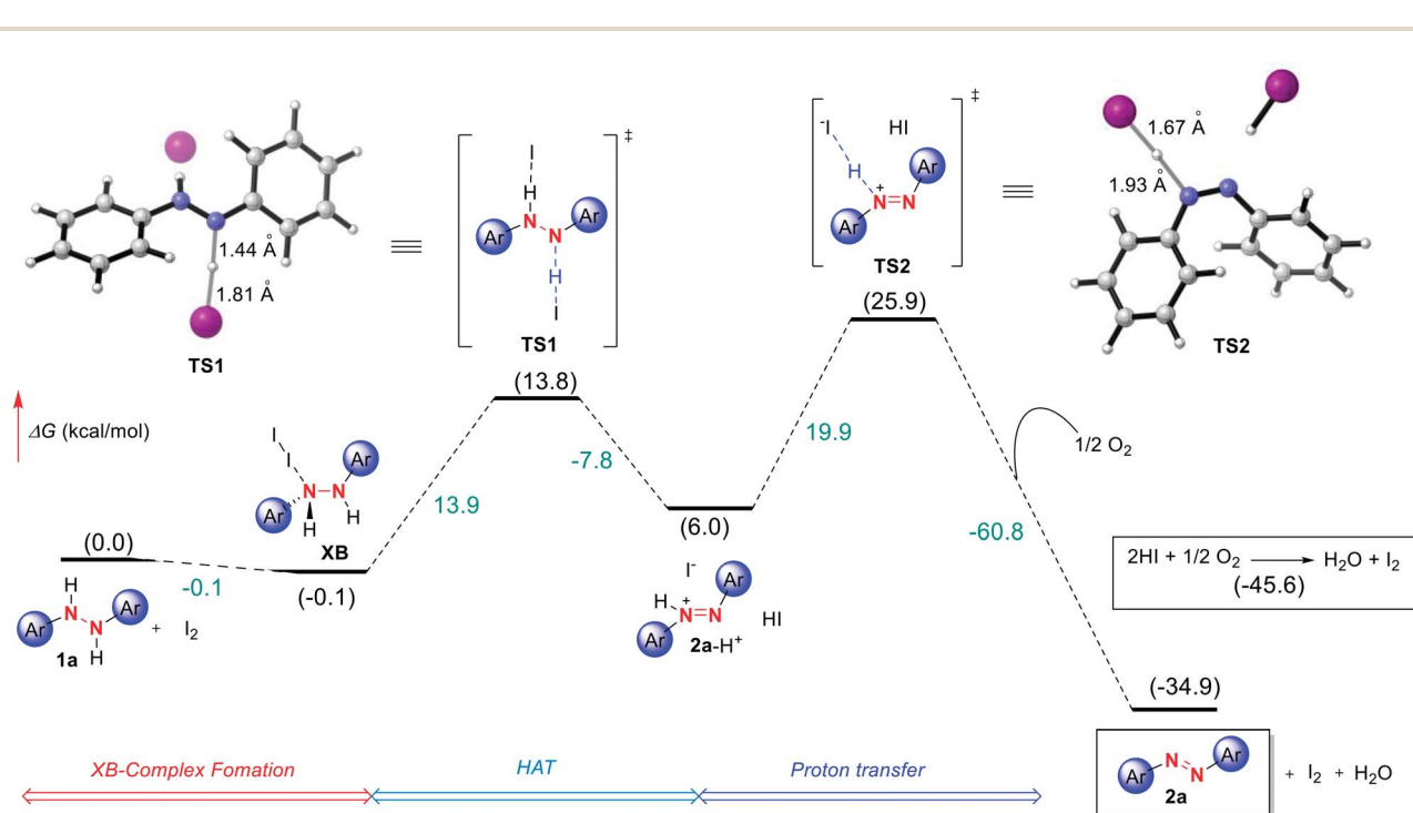
Fig. 3 Free energy profile for I 2 catalyzed azo formation computed at the (IEFPCM DCM )UAPFD/def2-TZVP//UAPFD/DGDZVP level of theory. Free energies are given in kcal mol -1 .
