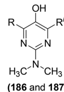
186; R = R' = -H ( IC_{50} = 602 \mu M ) 187; R = R' = -CH 3 ( IC_{50} = 593 \mu M )
