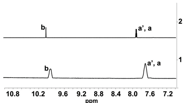
Fig. 2 Line 1: ^1\text{H} NMR spectra of 1-OH 2 * (2 mM) in the presence of PPI (10 equiv.; 20 mM; incubation time: 30 min) at pD 7.35 ( \text{D}_2\text{O} , [Tris buffer] = 10 mM). Line 2: ^1\text{H} NMR spectra of pure signaling aldehyde 4 in \text{D}_2\text{O} . Characteristic protons are indicated in Fig. 1A. * The ^1\text{H} NMR spectrum of 1-OH 2 did not show any signal in this region due to the paramagnetism of the probe.
