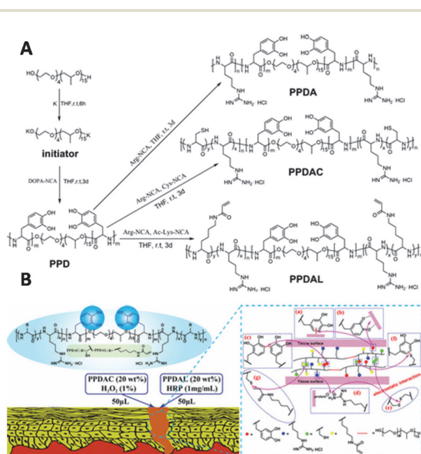
Fig. 27 A. Synthesis of PPDA (from L -arginine NCA), PPDAC (from L -cysteine NCA) and PPDAL (from \epsilon - N -acryloyl lysine-NCA) polypeptides. Reprinted from ref. 158 with permission from American Chemical Society, copyright (2017). B. Schematic representation of polymer interactions with skin substrate. Reprinted from ref. 158 with permission from American Chemical Society, copyright (2017).
