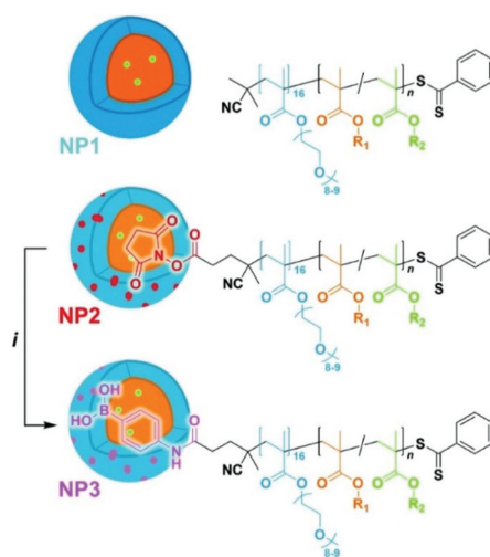
Fig. 6 Schematic illustration of the POEGM 0 - b -poly(4-pinacolboronyl-benzyl methacrylate). R 1 = 4-phenylboronate pinacol ester, R 2 = fluor-escen. Reproduced from ref. 26 with permission from the Royal Society of Chemistry, copyright 2020.
