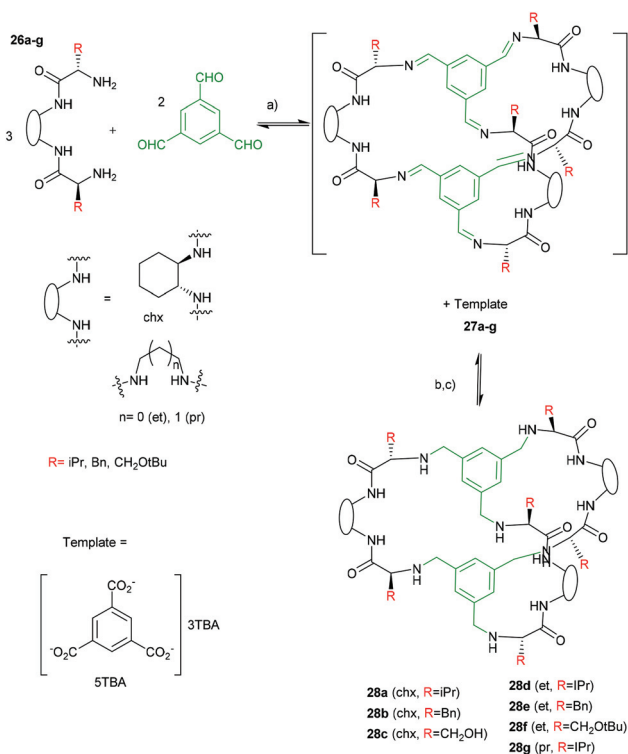
Scheme 1 Synthesis of pseudopeptidic cages described by Alfonso. 98 (a) Equilibrium at RT either in the absence or the presence of 5TBA. (b) \text{BH}_3 \cdot \text{py} (c) \text{HCl} .
