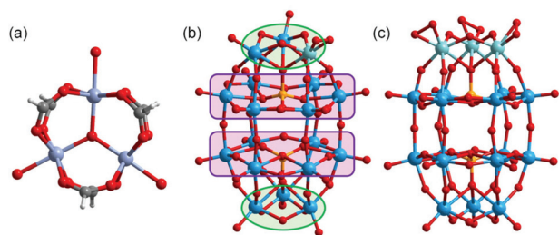
Fig. 1 Molecular structures of (a) [Cr_3O(OOCH)_6(H_2O)_3]^+ , (b) [P_2W_{17}(NbO_2)O_{61}]^{7-} and (c) [P_2W_{15}(MO_2)_3O_{59}]^{9-} (M = Nb or Ta). Color codes: W: blue; Nb or Ta: cyan; P: orange; O: red; Cr: silver; C: grey, and H: light grey. W atoms at the polar and equatorial sites of the Dawson-type POMs are surrounded by the green ovals and purple rectangles, respectively. W atoms at the polar sites are substituted with Nb or Ta atoms.
