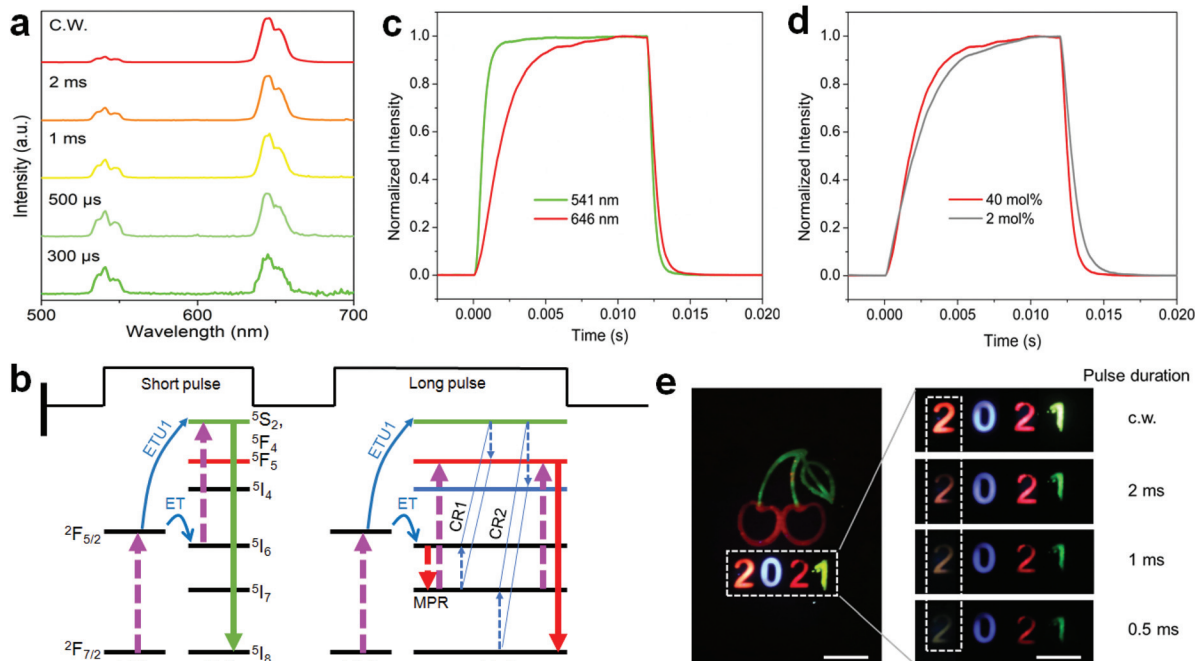
Fig. 7 (a) Upconversion emission spectra of \text{NaYF}_4:Ho(40 \text{ mol}\%)@NaYF_4:Yb(60 \text{ mol}\%)@NaYF_4 core–shell–shell nanoparticles under pulsed 980 nm excitation with a tuning of the pulse duration. (b) Schematic of the possible processes for the reduction of the red upconversion under non-steady state excitation. (c) Time-dependent emission profiles of \text{Ho}^{3+} at 541 and 646 nm of (a) sample under 980 nm irradiation with a pulse duration of 12 ms (50 Hz). (d) A comparison of the time-dependent red upconversion emission profiles from the (a) sample and \text{NaYF}_4:Yb/Ho(20/2 \text{ mol}\%)@NaYF_4 core–shell nanoparticles. (e) Schematic of decoding the concealed information on the cherry pattern under pulsed 980 nm irradiation (right panels) in which only the initial number “2” shows a color change with reducing the pulse duration. Scale bars, 0.5 cm.
