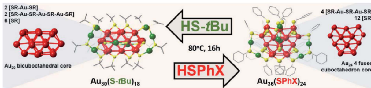
Fig. 17 Schematic of the conditions for the interconversion between \text{Au}_{30}(\text{S}^t\text{Bu})_{18} and \text{Au}_{36}(\text{SPhX})_{24} . Reaction takes place under the same thermochemical conditions with different thiol ligands (thiophenol and tert -butyl). Left panel: crystal structure of \text{Au}_{30}(\text{S}^t\text{Bu})_{18} , right panel: crystal structure of \text{Au}_{36}(\text{SPhX})_{24} . Color code: Au core atom: red, Au staple atom: green, sulphur: yellow, carbon: gray. Hydrogen atoms have been eliminated for clarity. Adapted with permission from ref. 125. Copyright 2017 American Chemistry Society.
