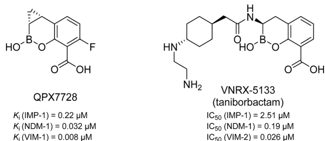
Fig. 1 Chemical structures and reported K_i/\text{IC}_{50} values against different MBLs of QPX7728 20,21 and VNRX-5133 (taniborbactam), 22–24 two cyclic boronates that are in clinical trials.
