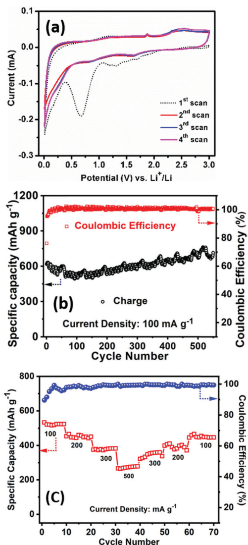
Fig. 5 Electrochemical half-cell LIB anode performance of the PSCNs. (a) Cyclic voltammetry of the PSCN electrode for the first four cycles at 0.1 mV s -1 at 0.01–3.0 V, (b) cycling performance at 100 mA g -1 current density, and (c) rate performance at different current densities (100–500 mA g -1 ).
