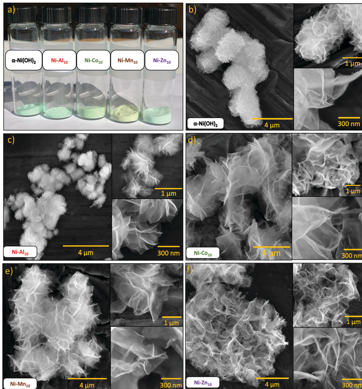
Fig. 1 (a) Photograph of microwave-synthesized powders—25 mg each of unsubstituted \alpha -Ni(OH) _2 , aluminum-substituted (Ni-Al _{10} ), cobalt-substituted (Ni-Co _{10} ), manganese-substituted (Ni-Mn _{10} ), and zinc-substituted (Ni-Zn _{10} ) nanosheets; (b–f) scanning electron micrographs of microwave-synthesized nanosheets at three different magnifications (6500 \times , 25 000 \times , 100 000 \times ); (b) unsubstituted \alpha -Ni(OH) _2 nanosheets, (c) aluminum-substituted nanosheets (Ni-Al _{10} ); (d) cobalt-substituted nanosheets (Ni-Co _{10} ); (e) manganese-substituted nanosheets (Ni-Mn _{10} ); and (f) zinc-substituted nanosheets (Ni-Zn _{10} ).
