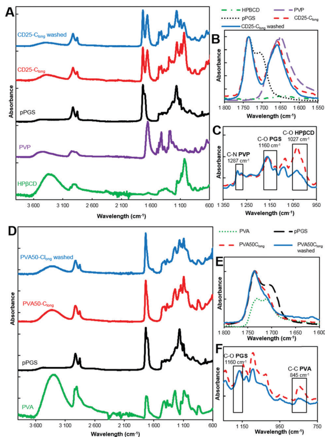
Fig. 4 ATR-FTIR spectra of CD25 (A–C) and PVA50 (D and E) after curing and after purification compared to HPβCD, PVP, PVA and corresponding pPGS spectra. (A and D) Full spectra, absorbance normalized to the 1730 \text{cm}^{-1} band. (B and E) C=O bands, absorbance normalized to the 1730 \text{cm}^{-1} band. (C and F) C–O, C–C and C–N bands, absorbance normalized to the 1160 \text{cm}^{-1} band.
