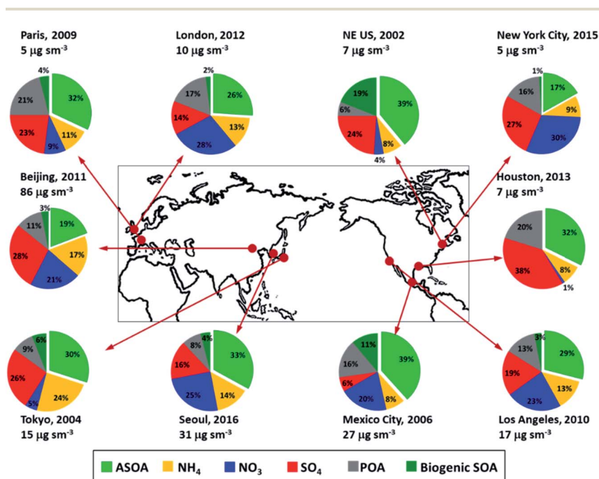
Fig. 3 Non-refractory submicron composition measured in urban and urban outflow regions from field measurements, all in units of μg m -3 at standard temperature (273 K) and pressure (1013 hPa) (adapted from Nault et al. 69 ).
