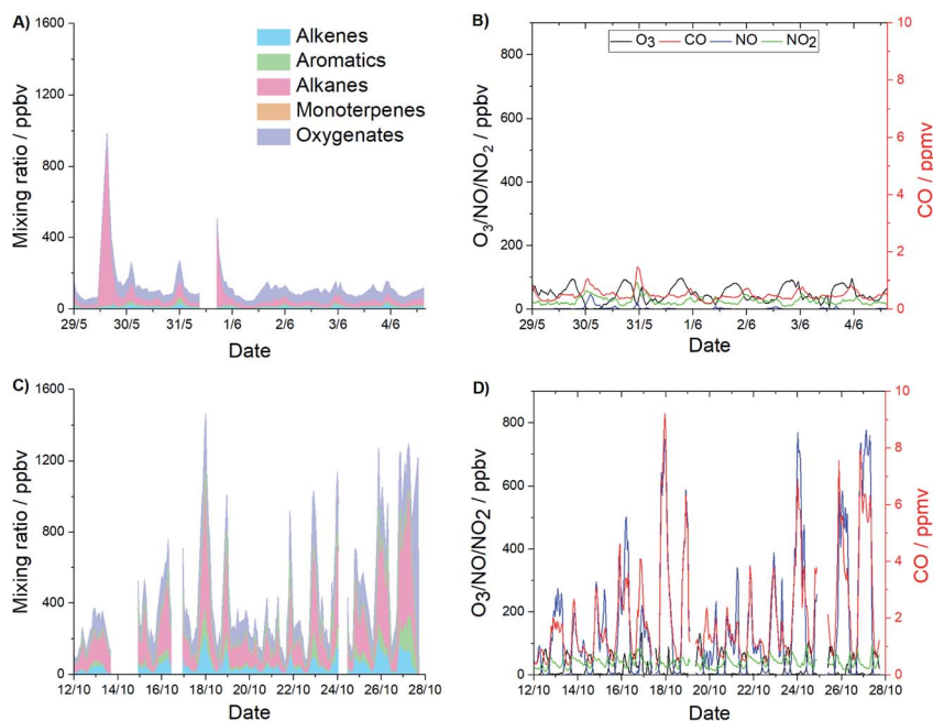
Fig. 4 Concentration–time series of (A) pre-monsoon NMHCs (stacked), (B) pre-monsoon O_3 , NO , NO_2 and CO , (C) post-monsoon NMHCs (stacked) and (D) post-monsoon O_3 , NO , NO_2 and CO . Zoomed in versions for the pre-monsoon campaign are available in the ESI10.†
