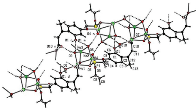
Fig. 5 X-ray structure of 2a trisodium 3-[4-(ethoxy-phosphonomethoxy)-2-phenolato]-but-2-enoate trihydrate. Left: showing \text{Na}^+\cdots\text{O}-\text{P} , \text{Na}^+\cdots\text{O}-\text{C} and \text{Na}^+\cdots\text{OH}_2 bonding. Right: the extended hydrogen bonded chain structure.
