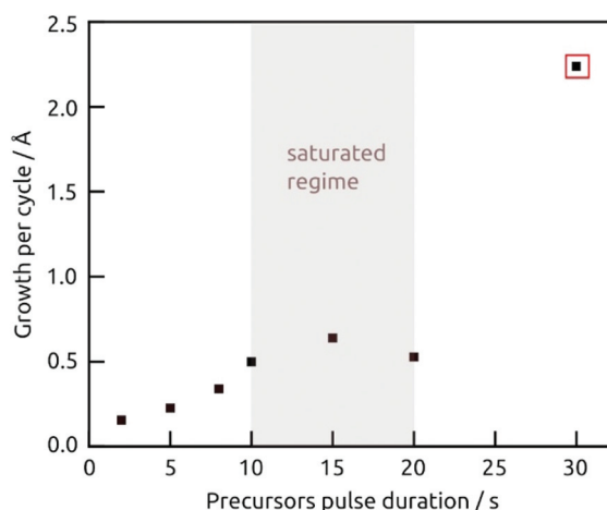
Fig. 3 Growth rate as a function of the precursors pulse duration, the concentrations for \text{Hf}(\text{NMe}_2)_4 and \text{H}_2\text{S} are 1 mM and 2 mM, respectively, and the solvent purging is 60 s for each half cycle. Note that the thickness for the marked data point was measured after removing the dusty precipitate with sonication in hexane.
