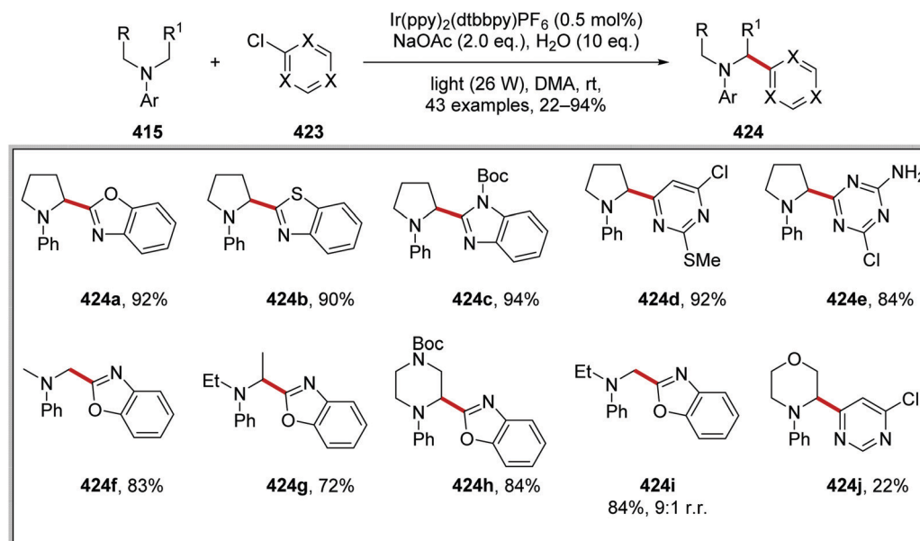
Scheme 118 Results of coupling between heteroaryl chlorides 423 and alkanilines 415 .
