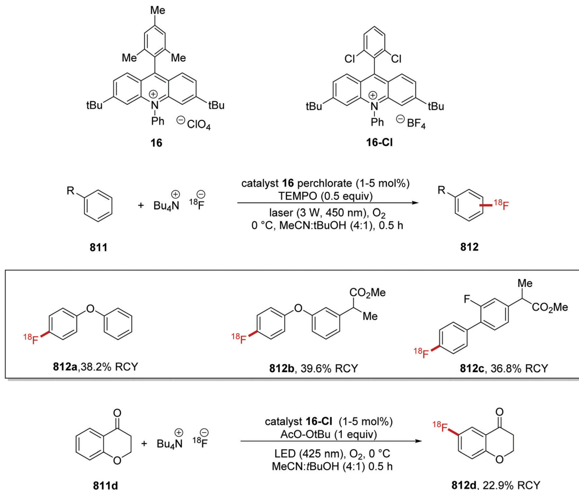
Scheme 222 C–H radiofluorination of arenes.
