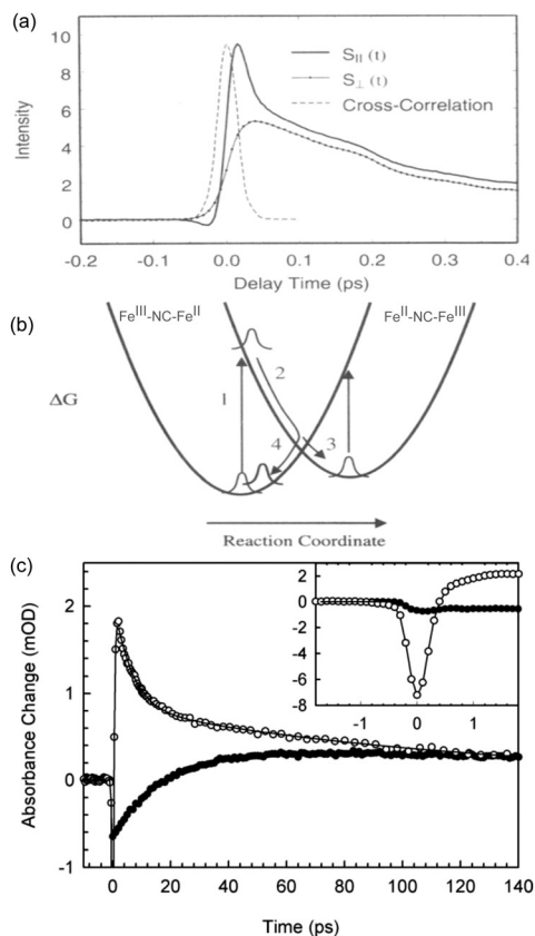
Fig. 3 Ultrafast dynamics in Fe-Fe PB. (a) The early 50 fs dynamics in the polarisation dependent transient transmission of FeFe PB shows a difference between the parallel ( S_{\parallel} ) and perpendicular ( S_{\perp} ) signals. (b) Model developed by Arnett et al. showing how either the excited CT state (2) can decay back to the groundstate ( 4 \rightarrow 1 ) or how a long-lived CT state (3) could be formed. (a) and (b) are reprinted with permission from Arnett et al. J. Am. Chem. Soc. , 1995, 117 , 12262–12272. 122 Copyright 1995 American Chemical Society. (c) In an experiment by Weidinger et al. , ESA probed at 800 nm was identified after pumping at both 800 nm (open circles) and IR pulses resonant with the CN stretch mode (solid circles). After an initial bleach signal, the IR-pumped signal shows an ESA (positive signal). Figure reprinted from Weidinger et al. J. Chem. Phys. , 2011, 134 , 124510, 127 with the permission of AIP Publishing.
