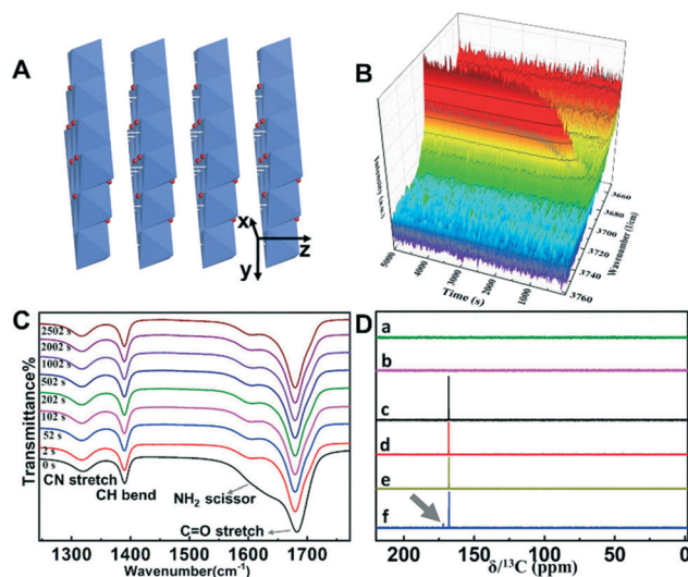
Fig. 4 (A) Atomic structure of \text{Co(OH)}_2 , \text{Fe(OH)}_2 , \text{Mn(OH)}_2 , \text{Zn(OH)}_2 , \text{Cu(OH)}_2 \cdot \text{H}_2\text{O} and \text{Mg(OH)}_2 . (B) Evolution of the typical O–H stretching mode of the Mg–OH groups over time. (C) FTIR spectra of the reaction process after introducing \text{NH}_3 into the formamide aqueous solution containing \text{MgCl}_2 in the 1000\text{--}2000\text{ cm}^{-1} region. (D) ^{13}\text{C} NMR spectra of (a) pure water after introducing \text{NH}_3 , (b) aqueous solution containing \text{MgCl}_2 after introducing \text{NH}_3 , (c) pure formamide aqueous solution, (d) formamide aqueous solution containing \text{MgCl}_2 , (e) formamide aqueous solution after introducing \text{NH}_3 without \text{MgCl}_2 and (f) formamide aqueous solution containing \text{MgCl}_2 after introducing \text{NH}_3 .
