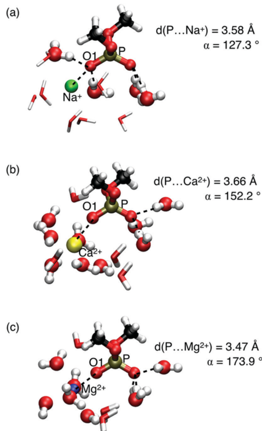
Fig. 8 DMP( \text{H}_2\text{O} ) _N\text{M}^{x+} cluster geometries ( \text{M}^{x+} = \text{Na}^+, \text{Mg}^{2+} , N = 11 ; \text{M}^{x+} = \text{Ca}^{2+} , N = 13 ). Water molecules of the first hydration shell around the ions and hydrogen bonded water molecules with DMP in ball-and-stick representation; the O1 atom of the (\text{PO}_2)^- group replaces one of the water oxygen atoms in the octahedral solvation geometry around the \text{Mg}^{2+} ion. Vibrational frequencies \nu_{\text{AS}}(\text{PO}_2)^- of structures shown in a, b and c are 1208, 1226, and 1248 \text{cm}^{-1} , respectively. Adapted with permission from ref. 65. Copyright 2019 American Chemical Society.
