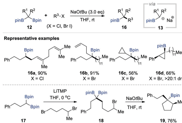
Scheme 4 NaOtBu-mediated deborylative alkylation of gem -bis[(pinacolato)boryl]alkanes.
