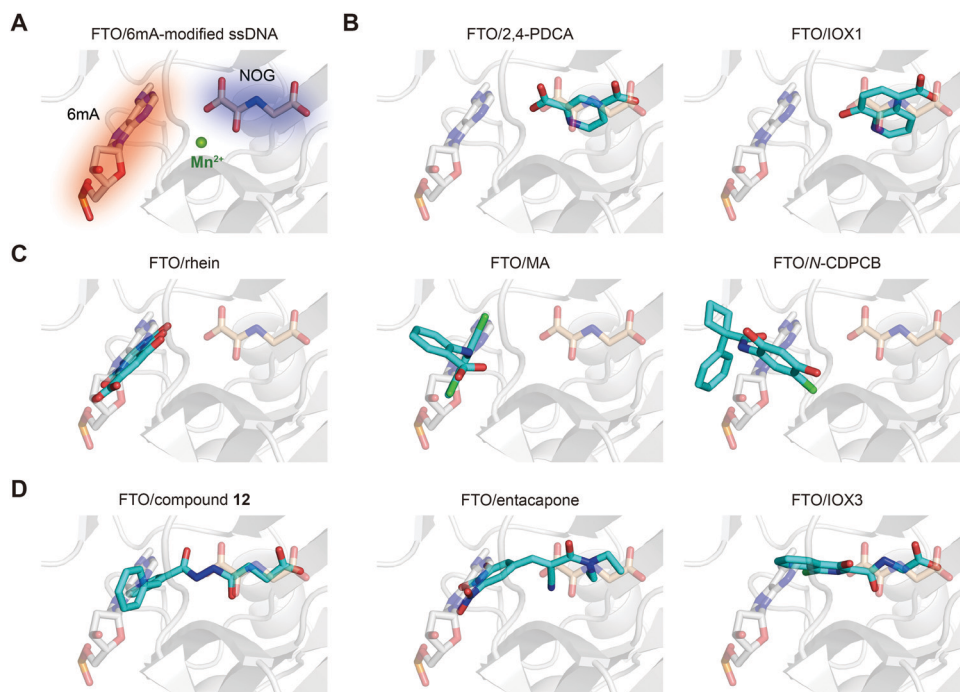
Fig. 7 The binding poses of representative FTO inhibitors. (A) The 6mA substrate (grey stick) and NOG (wheat stick) form two binding sites for chemical intervention (PDB: 5ZMD). Mn 2+ is shown as a green sphere. (B) Representative 2OG-competitive FTO inhibitors 2,4-PDCA (PDB: 4IE0) and IOX1 (PDB: 4IE4). (C) Representative substrate-competitive FTO inhibitors rhein (PDB: 4IE7), MA (PDB: 4QKN) and N-CDPCB (PDB: 5DAB). (D) Representative binding poses of both 2OG- and substrate-competitive FTO inhibitors compound 12 (PDB: 4CXW), entacapone (PDB: 6AK4) and IOX3 (PDB: 4IE6). All inhibitors are coloured cyan.
