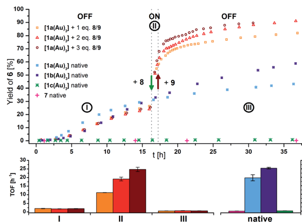
Fig. 4 (Top) Yield-over-time graphs for native (crossed symbols) and redox-switchable (hollow symbols) gold(I)-catalysed cyclisation of 5 to 6 (2 mol% Au as [\mathbf{1a}(\text{Au})_3] and 7 , [\mathbf{5}]_0 = 60 \text{ mmol L}^{-1} , \text{CD}_2\text{Cl}_2 , 25^\circ\text{C} ). Arrows indicate the addition of additives. I: initial OFF phase with little catalytic activity; II: ON phase after addition of 1.0–3.0 eq. oxidant 8 ; III: 2 nd OFF phase of little catalytic activity after addition of 1.1–3.3 eq. reductant 9 . (Bottom) Comparison of turnover frequencies (TOF), determined from linear fits of fixed time frames (s. Fig. S39–S45 † ) for the switched reaction phases shown above (left) and for the native complexes (right).
