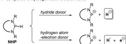
c) Consumption and regeneration of the catalyst NHP
