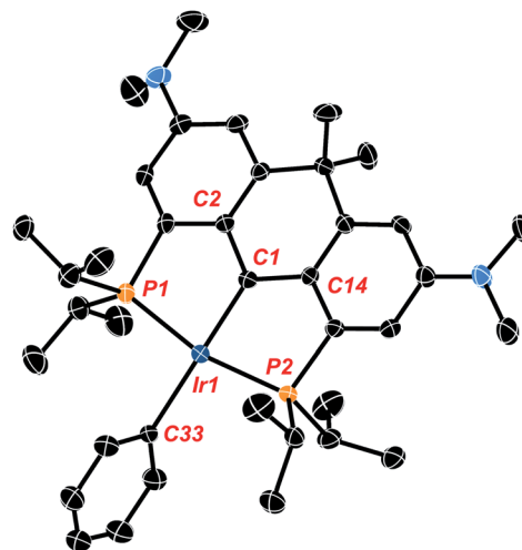
Fig. 2 Synthesis and thermal ellipsoid diagram of Ir-Ph (ellipsoids drawn to 50% probability; hydrogen atoms have been omitted for clarity). Selected metrical data for Ir-Ph: bond distances (Å): Ir1–C1, 1.965(4); Ir–C33, 2.118(4); Ir1–P1, 2.2581(13); Ir1–P2, 2.2671(17), C1–C2, 1.467(6); C1–C14 1.469(6). Bond angles (°): P1–Ir1–P2, 166.46(4); C1–Ir1–C33, 179.53(19); P1–Ir1–C1, 83.46(13); P1–Ir1–C33, 96.38(13); Ir1–C1–C2, 122.6(3); Ir1–C1–C14, 122.9(4); C2–C1–C14, 114.5(4).
