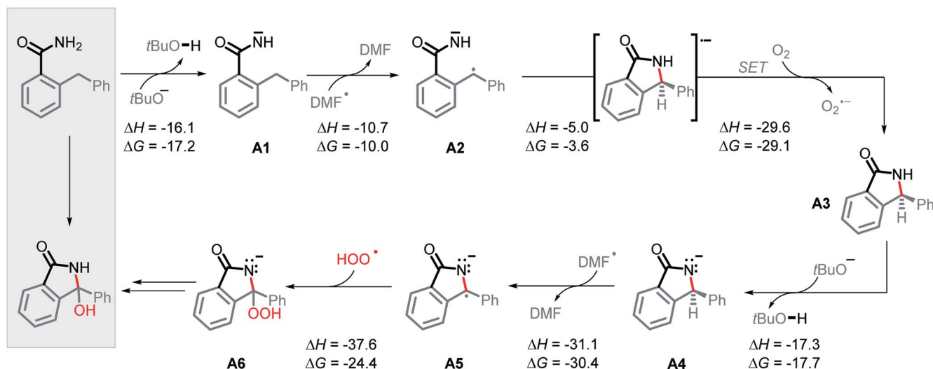
Scheme 6 Proposed mechanism and calculated reaction thermodynamics for the N-H/C-H amidation. All energies are in kcal mol -1 .
