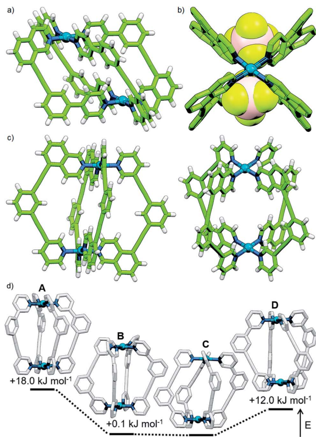
Fig. 5 Solid state structure of cis\text{-}[\text{Pd}_2(\mathbf{2})_4](\text{BF}_4)_4 viewed (a) from the side and (b) down the Pd-Pd axis with encapsulated \text{BF}_4^- anions shown (hydrogen atoms omitted for clarity). Bond lengths (Å): Pd-N pyridine 1.990(17)/2.069(2); Pd-N isoquinoline 2.029(3)/2.040(3). (c) Solid state structure of cis\text{-}[\text{Pd}_2(\mathbf{4})_4](\text{BF}_4)_4 . Bond lengths (Å): Pd-N pyridine 2.044(8)/2.056(8); Pd-N isoquinoline 2.006(9)/2.007(8). (d) Calculated structures (B3LYP/6-31G(d)/SDD) of the A, B, C and D isomers of [\text{Pd}_2(\mathbf{5})_4]^{4+} with energies relative to C. Hydrogen atoms have been omitted for clarity.
