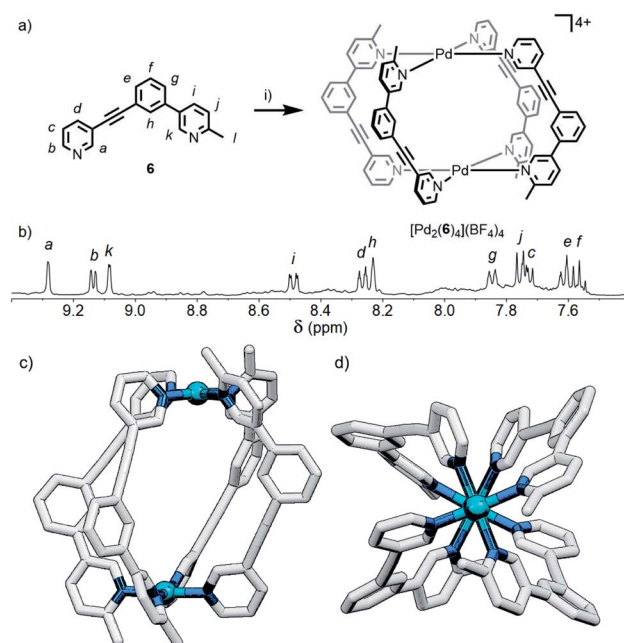
Fig. 6 (a) Formation of the cis\text{-Pd}_2\text{L}_4 cage [\text{Pd}_2(\mathbf{6})_4](\text{BF}_4)_4 . Reagents and conditions: (i) [\text{Pd}(\text{CH}_3\text{CN})_4](\text{BF}_4)_2 , d_6\text{-DMSO} , rt, 24 h. (b) Partial 1 H NMR spectrum (400 MHz, 298 K, d_6\text{-DMSO} ) of [\text{Pd}_2(\mathbf{6})_4](\text{BF}_4)_4 . Calculated structure (B3LYP/6-31G(d)/SDD) of cis\text{-}[\text{Pd}_2(\mathbf{6})_4]^{4+} viewed from (c) the side, and (d) down the Pd-Pd axis; hydrogen atoms have been omitted for clarity.
