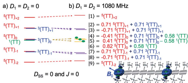
Fig. 4 Schematic representation of the sublevels of SCTP, as the weakly coupled multiexciton in (b) caused by the ZFS interactions ( D_1 = D_2 = 1080 \text{ MHz} ) of ^3\text{TIPS-Pn} . The energy shifts in the SCTP levels in (b) are shown with respect to the levels in (a) with D_1 = D_2 = 0 in the presence of the external magnetic field (340 mT) for highly separated T + T ( D_{\text{SS}} = 0 and J = 0 ). The wavefunctions were computed for the field direction ( \mathbf{B}_0 ) parallel to the out-of-plane axes of the aromatic rings.
