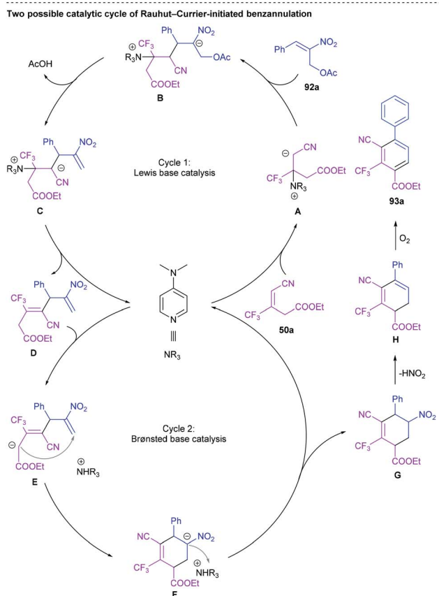
Scheme 26 DMAP-catalyzed [3 + 3] benzannulation to synthesize biaryls.
