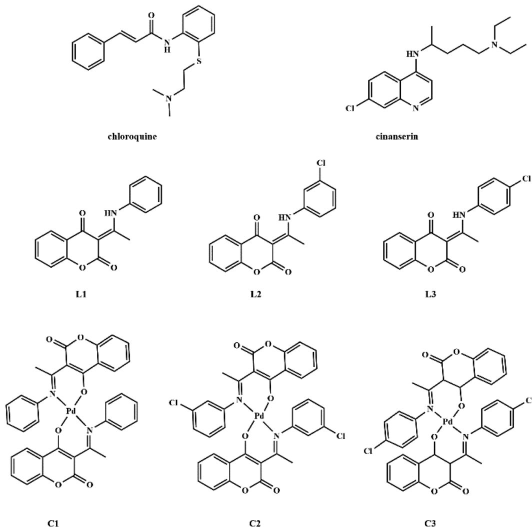
Fig. 1 Structures of chloroquine, cinanserin, coumarine derivatives and their palladium(II) complexes.
