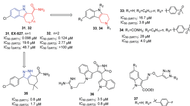
Fig. 6 Chemical structures of indole-based SIRT2 inhibitors and their inhibitory activity data on SIRTs by isotope labelling, Sirt-Glo™ assay kit 50 or fluorescence-based assays. 51
