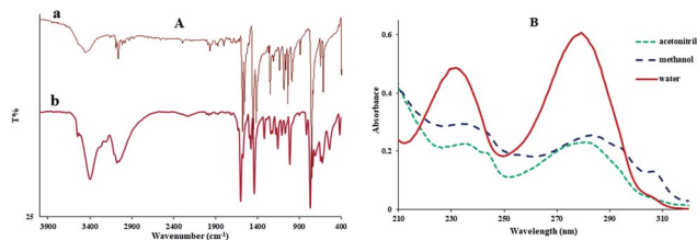
Fig. 1 (A) FT-IR spectra of (a) 2,2'-bipyridine ligand, (b) Sm complex. (B) The UV-vis spectra of the Sm-complex in different solvents ([Sm-complex] = 1 \times 10^{-5} \text{ M} ).
