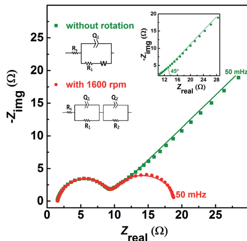
Fig. 2 EIS patterns recorded at EP on carbon-modified GCE without rotation and with 1600 rpm in equimolar (0.2 M) concentration of \text{V}^{4+} and \text{V}^{5+} in 3 \text{ M H}_2\text{SO}_4 electrolyte. The symbols and solid lines show the experimental and the fitted data, respectively. The corresponding ECs are shown in the insets. The expanded view of the 45^\circ line is shown in the inset.
