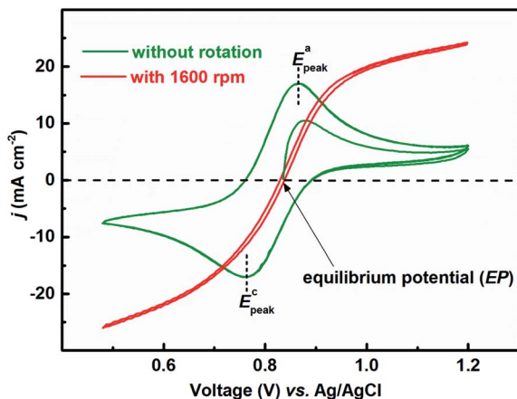
Fig. 1 CVs recorded with carbon-modified GCE without rotation and with 1600 rpm at 20 \text{ mV s}^{-1} scan rate in equimolar (0.2 M) concentration of \text{V}^{4+} and \text{V}^{5+} in 3 \text{ M H}_2\text{SO}_4 electrolyte.
