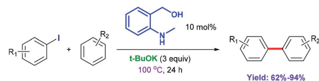
Scheme 1 Synthesis of biaryls and their derivatives from aryl halides and unactivated arenes.
