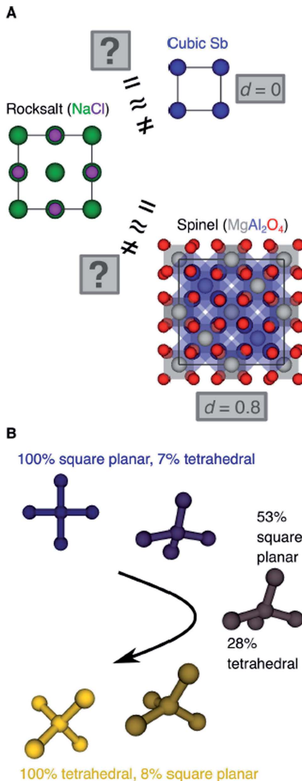
Fig. 2 (A) Is rocksalt structurally (more) similar to cubic Sb or to MgAl_2O_4 -spinel? (B) Can we create descriptors which measure the degrees of resembling perfect coordination environments in a comparable way?
