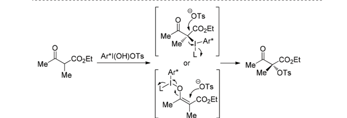
Scheme 52 Asymmetric oxidation of \alpha -substituted \beta -ketoesters promoted by C_2 -symmetric iodoarene.
