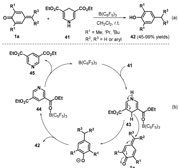
Scheme 11 \text{B}(\text{C}_6\text{F}_5)_3 -Catalyzed reduction of p -QMs.
