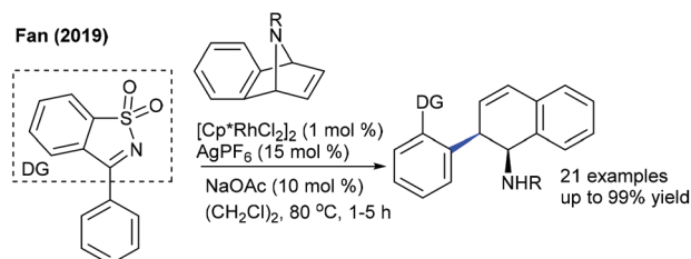
Scheme 80 Coupling of 7-azabenzonorbornadiene with N -sulfonyl ketimines.
