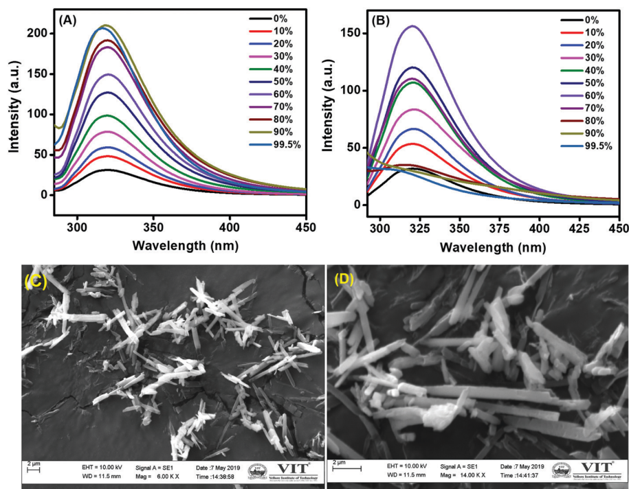
Fig. 3 Fluorescence spectra of 1 \times 10^{-5} M (A) L1 and (B) L2 in THF- \text{H}_2\text{O} with various water fractions. SEM images of (C) L1 (10%:90%, THF: \text{H}_2\text{O} ) and (D) L2 (40%:60%, THF: \text{H}_2\text{O} ).
