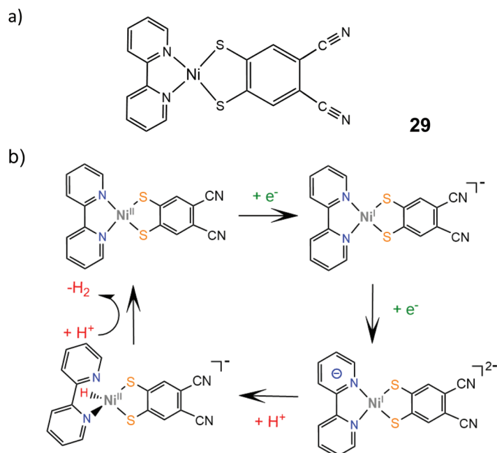
Scheme 17 (a) Molecular structure of Ni(bpy)(dcbdt). (b) Proposed EECC mechanism catalysed by complex 29.
