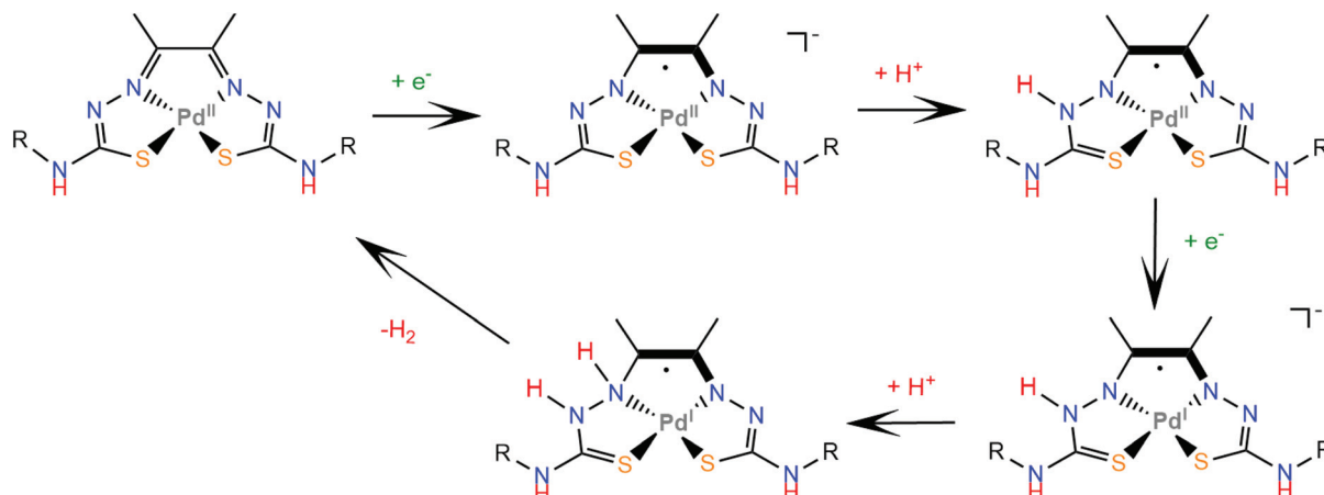
Scheme 32 Proposed ECEC mechanism catalysed by complex 69.
