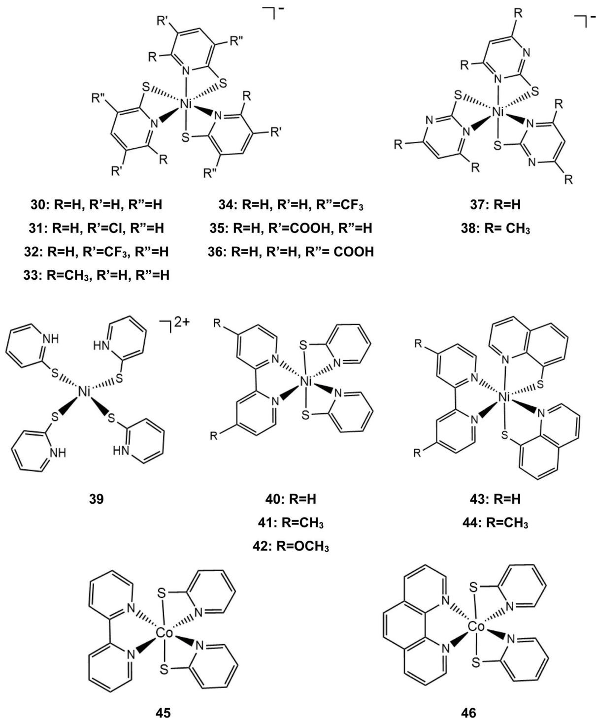
Scheme 18 Molecular structures of metal pyridine–thiolate HER catalysts.
