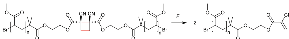
Scheme 2 Dicyano-substituted cyclobutane undergoing force-induced cycloelimination. 24
