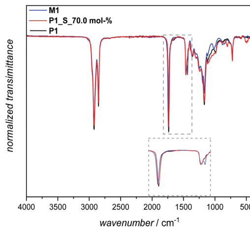
Fig. 4 Analysis of M1 , P1 and P1_S_70.0 mol% by attenuated total-reflectance infrared spectroscopy, indicating the success of each transformation, i.e. synthesis of the parent polymer P1 and the subsequent transformation into high sulfur content polyester P1_S_70.0 mol% . The inset shows the zoomed-up region from 1800–1400 \text{cm}^{-1} , respectively.
