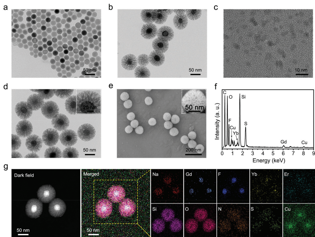
Fig. 1 Structural and compositional characterization of UMNOCC-PEG nanoparticles. TEM images of (a) the NaGdF 4 :Yb,Er core nanoparticles, (b) UCNP@dMSN-SNO, (c) Cu 2 O nanodots, and (d) UMNOCC-PEG nanoparticles. (e) SEM image and (f) corresponding EDS spectrum of the UMNOCC-PEG nanoparticles. (g) Dark-field STEM image and the corresponding elemental mappings of UMNOCC-PEG nanoparticles.
