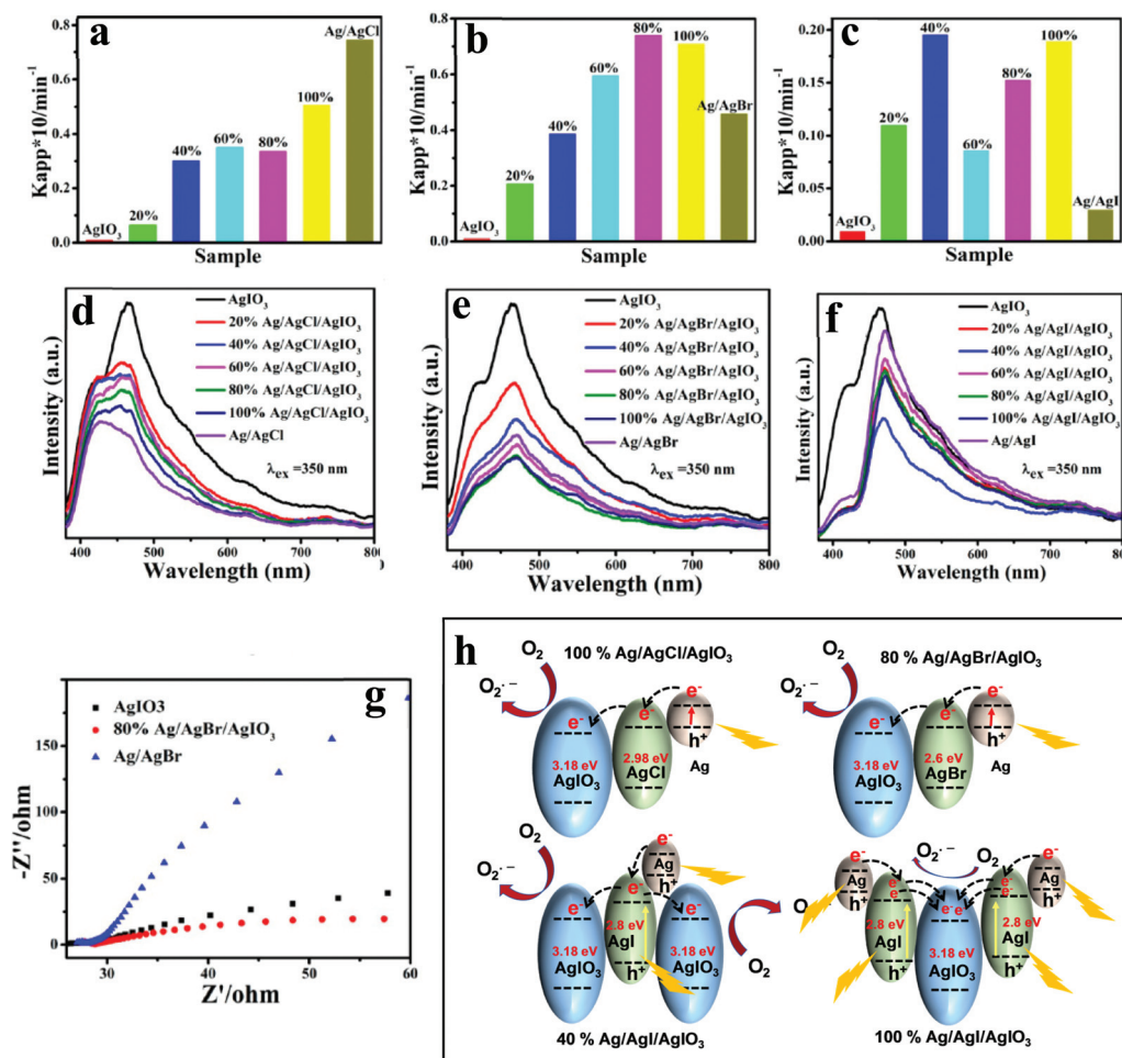
Fig. 8 Apparent rate constants for the photodegradation of MO over \text{AgI/O}_3 , \text{Ag/AgCl} , and \text{Ag/AgCl/AgI/O}_3 composites (a); \text{AgI/O}_3 , \text{Ag/AgBr} , and \text{Ag/AgBr/AgI/O}_3 (b); \text{AgI/O}_3 , \text{Ag/AgI} , and \text{Ag/AgI/AgI/O}_3 (c) under the irradiation of visible light, corresponding (d–f) PL spectra under an excitation of 350 nm, and (g) EIS Nyquist plot of \text{AgI/O}_3 , 80% \text{Ag/AgBr/AgI/O}_3 , and \text{Ag/AgBr} . (h) Schematic illustration of different charge-transfer mechanisms of 100% \text{Ag/AgCl/AgI/O}_3 , 80% \text{Ag/AgBr/AgI/O}_3 , 40% \text{Ag/AgI/AgI/O}_3 , and 100% \text{Ag/AgI/AgI/O}_3 . Fig. 6a–g: Copyright 2016, American Chemical Society. Reprinted from ref. 75 with permission.
