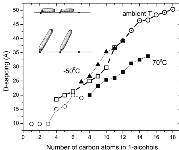
Fig. 3 Swelling of graphite oxide in 1-alkanols. The interlayer distance evaluated by XRD using d(001) vs. the number of carbon atoms in the alcohol molecule (1 for methanol, 2 for ethanol etc.). Open symbols are for data recorded in liquid solvents at ambient temperature (○- ref. 94; □- ref. 95). Ref. 95 provides also data for swelling at -50^{\circ}\text{C} (▲) recorded using frozen solid samples (except for octanol recorded in liquid) and at 70^{\circ}\text{C} (■). Inset shows the hypothetical change in orientation of alcohol molecules intercalated into the graphite oxide structure for larger alcohols. 98 The data points were copied from the published figures and are not precise.
