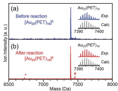
Fig. 2 MALDI mass spectra of [Au 25 (PET) 18 ] 0 (a) before and (b) after the HER experiment with twenty scans. The peaks indicated by asterisk (*) and hash (#) symbols are assigned to Au 23 (PET) 16 and Au 25 (PET) 18 S 2 , respectively, which are caused by laser irradiation.
