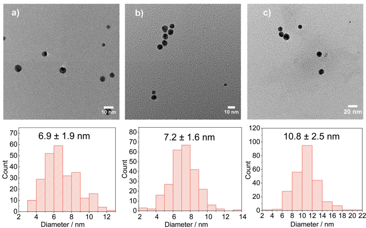
Fig. 8 Representative TEM images and particle size distribution of Au NPs synthesised using \text{AuCl} as precursor with a \text{DC}^{2-} : \text{Au} molar ratio of a. 20 : 1, b. 10 : 1 and c. 1 : 1. Conditions: [\text{AuCl}] : 0.25 mM, [\text{citrate}] : 5 mM, pH: 4.4, 80 °C, time: 7 min–11 min.
